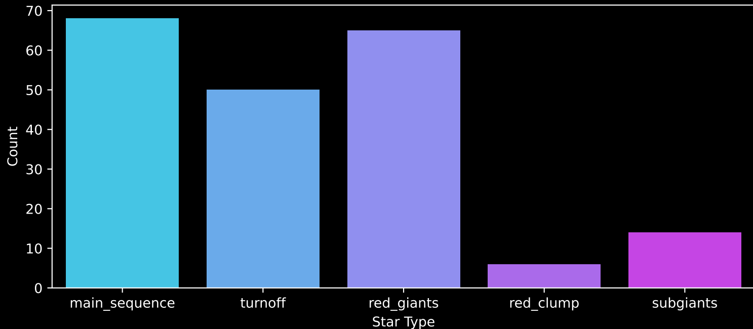
GALAH DR4 Field: [661] Count plot of Star Type
