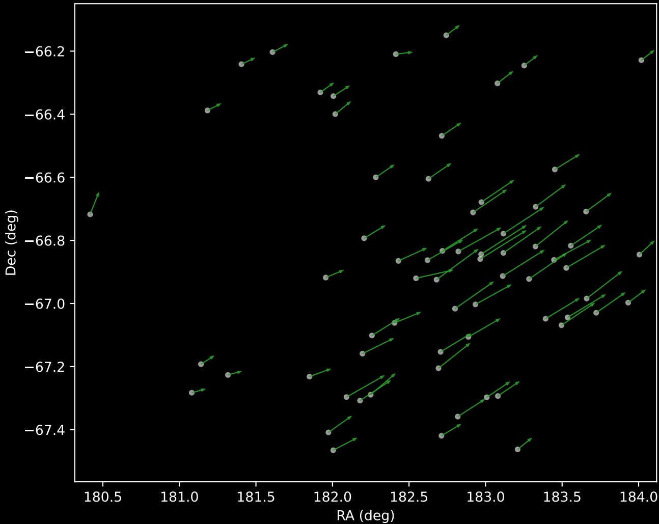
GALAH DR4 Cluster 4 Proper Motion Vectors (n=67)
