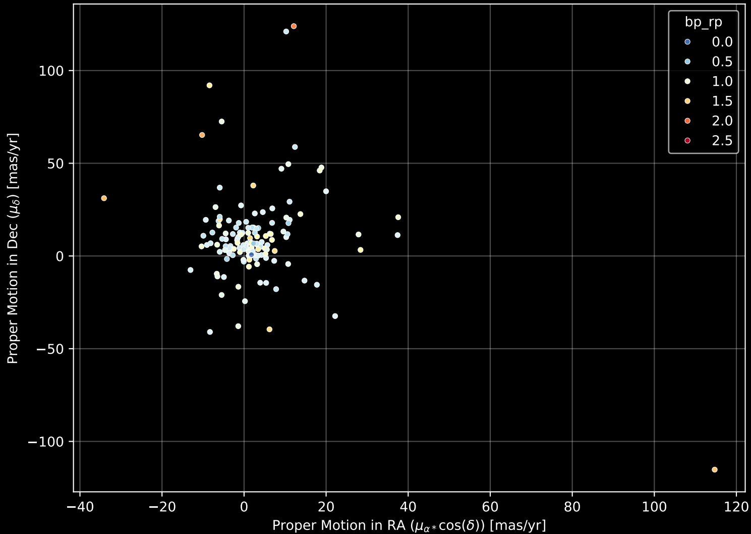
GALAH DR4 Field: [661] Proper Motion Diagram (n= 203)
