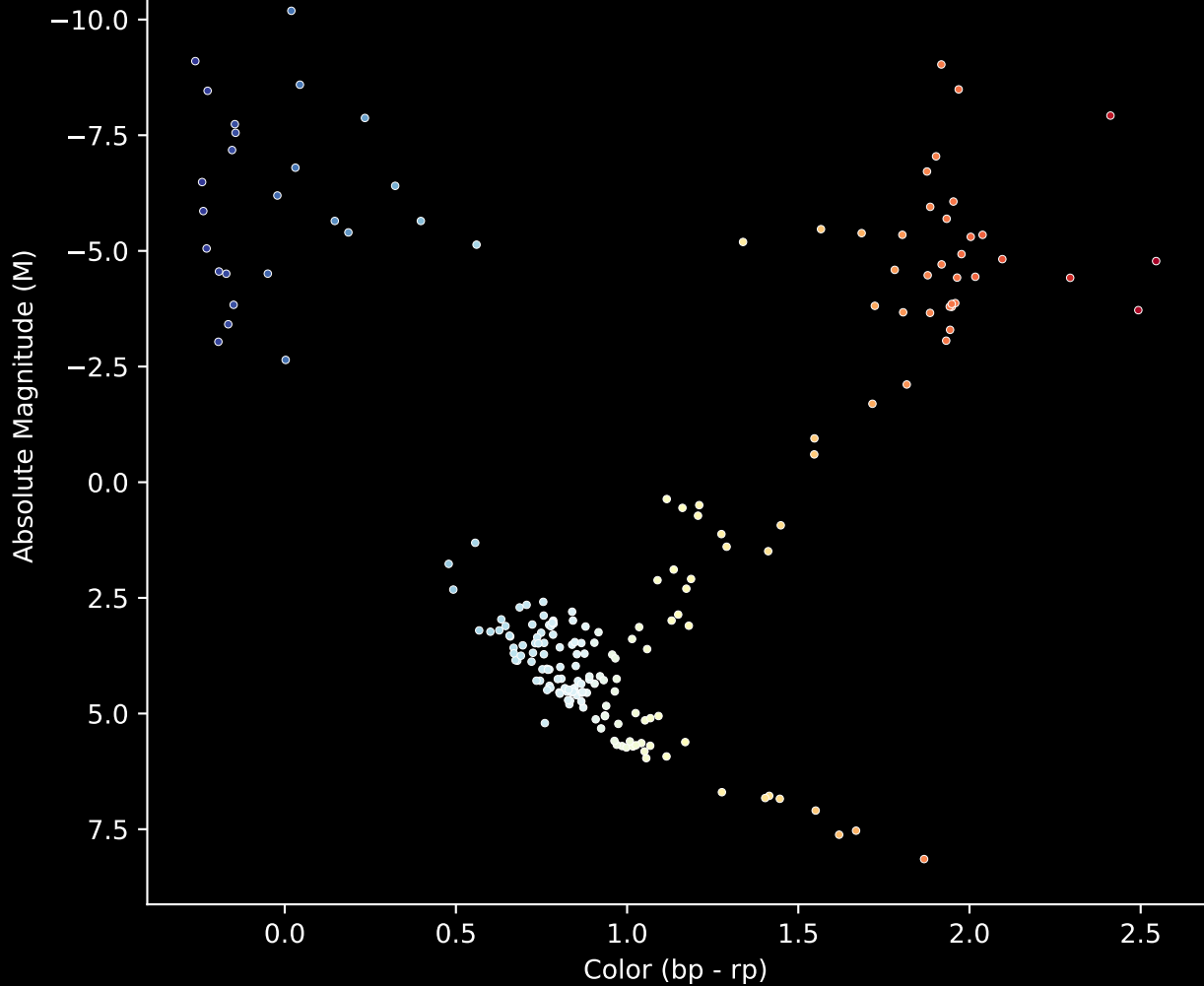
GALAH DR4 Field [661] Stars (n= 203) Hertzsprung-Russel Diagram
