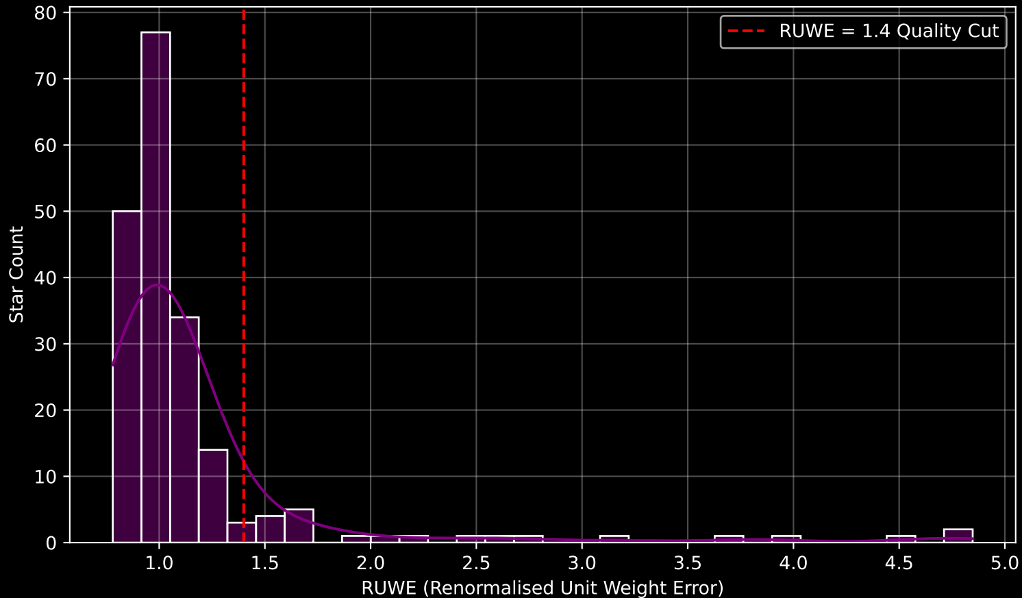
GALAH DR4 Field [661] RUWE Distribution (n= 199)
